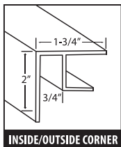
INSIDE/OUTSIDE CORNER
