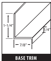
BASE TRIM
