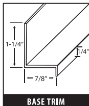
BASE TRIM
