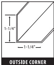
OUTSIDE CORNER
