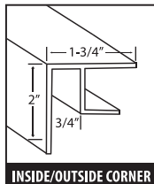
INSIDE/OUTSIDE CORNER
