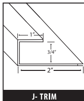
J-TRIM
