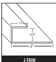
J-TRIM
