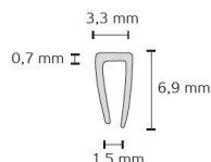
Top U-Profile
