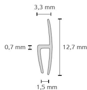
Connection Profile
